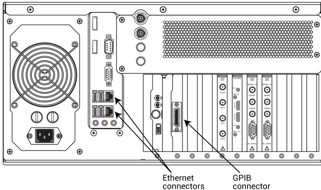
Figure 1: GPIB and ethernet connectors on the 4200A-SCS
