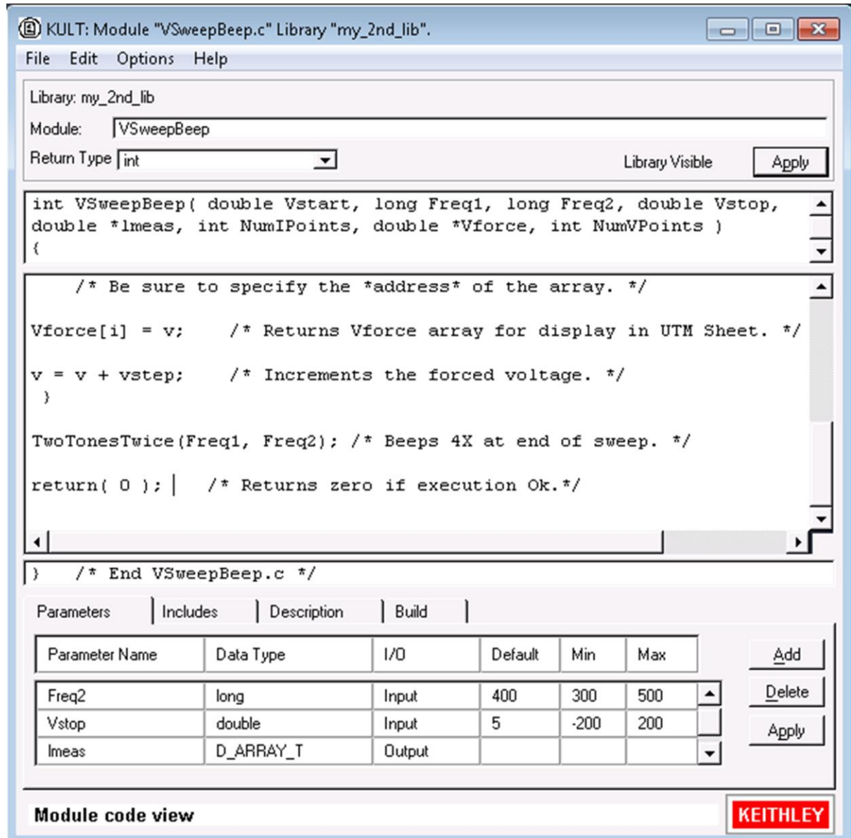
Figure 25: Completed VSweepBeep user module
