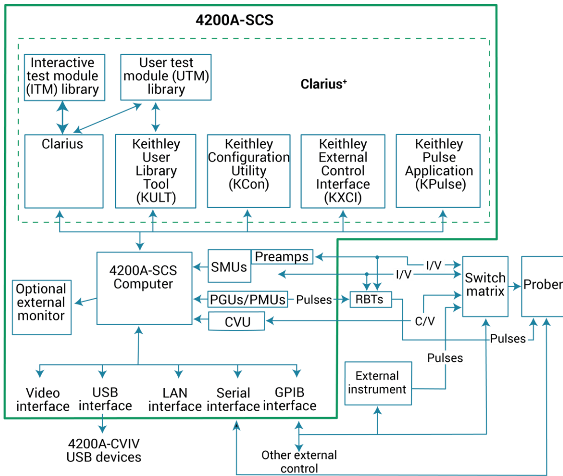
Figure 1: 4200A-SCS summary
