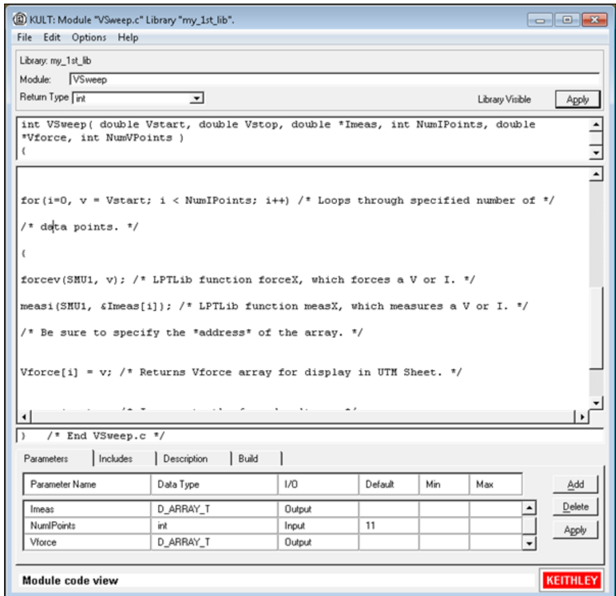
Figure 21: VSweep user-module dialog box after entering and applying code and parameters
