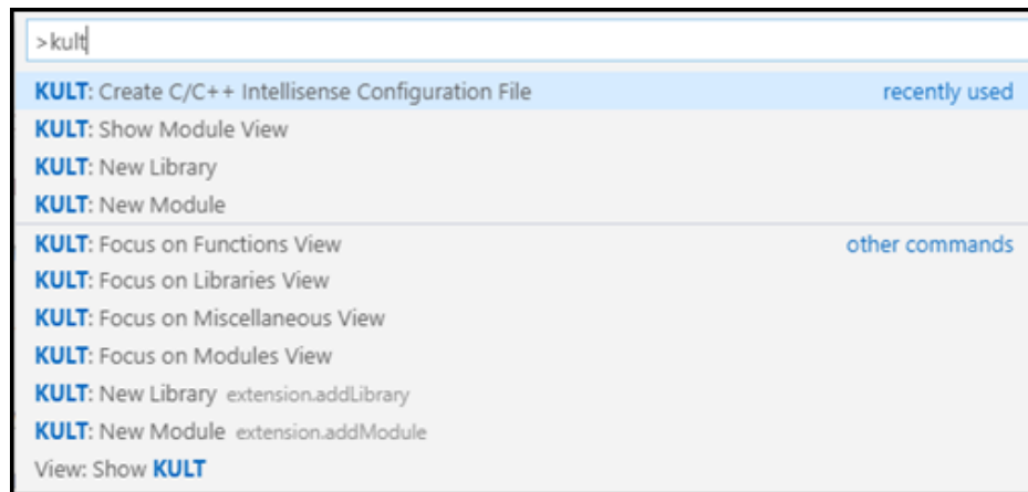
Figure 62: Command Palette
