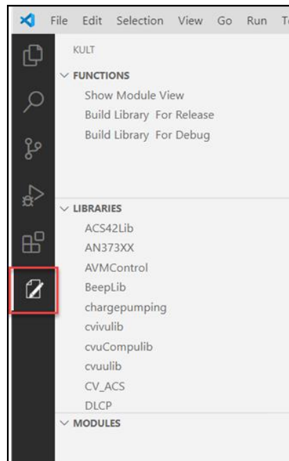
Figure 90: Opening the KULT side bar in Visual Studio Code
