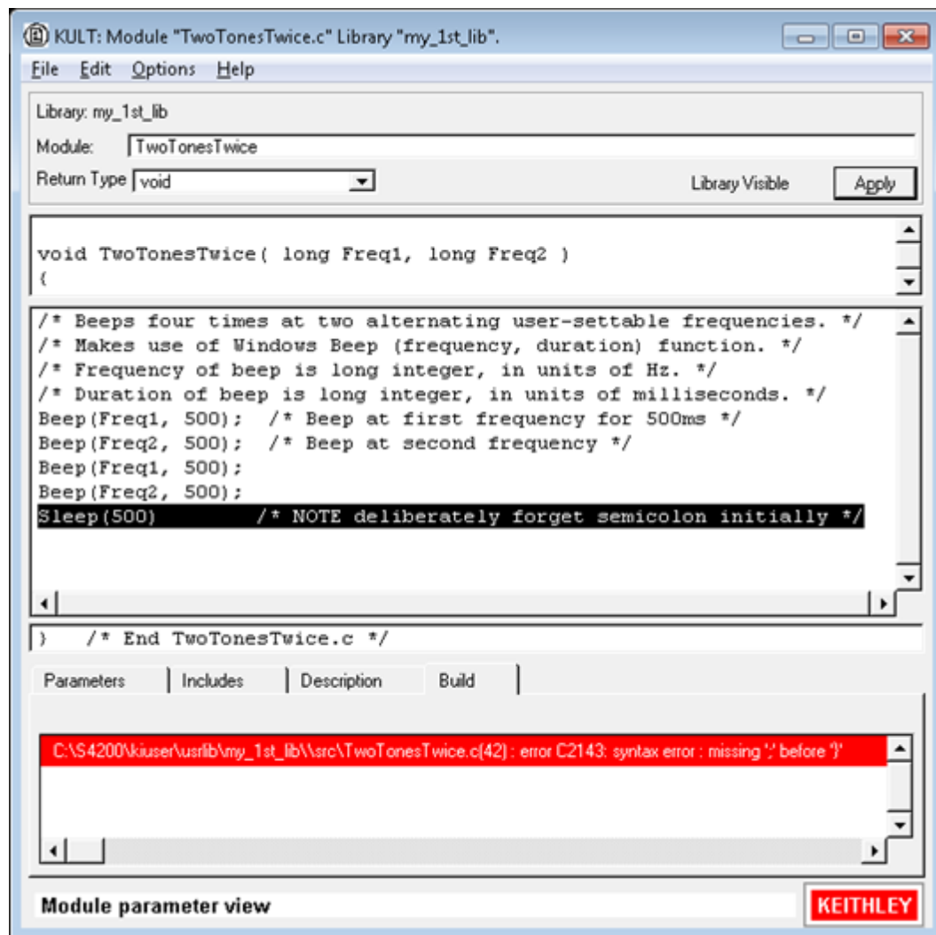
Figure 17: Find a code error
