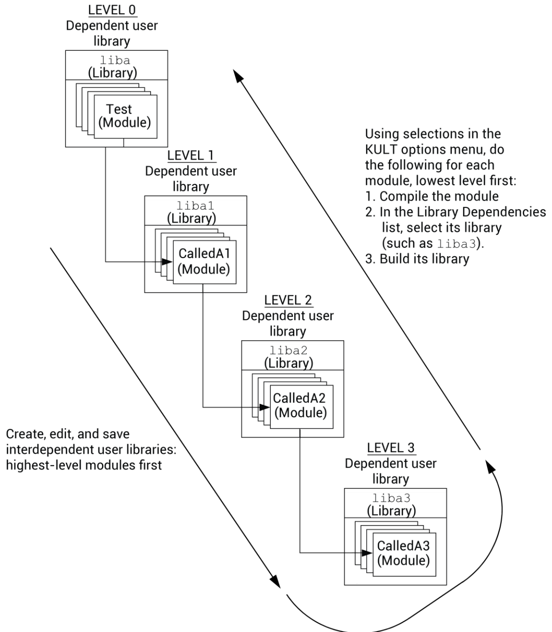
Figure 35: Hierarchical design for user library dependencies
