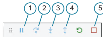
Figure 88: Debug toolbar
