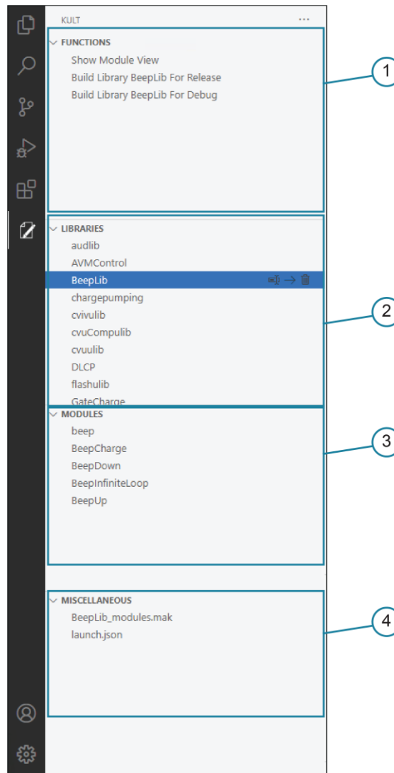
Figure 64: KULT side bar
