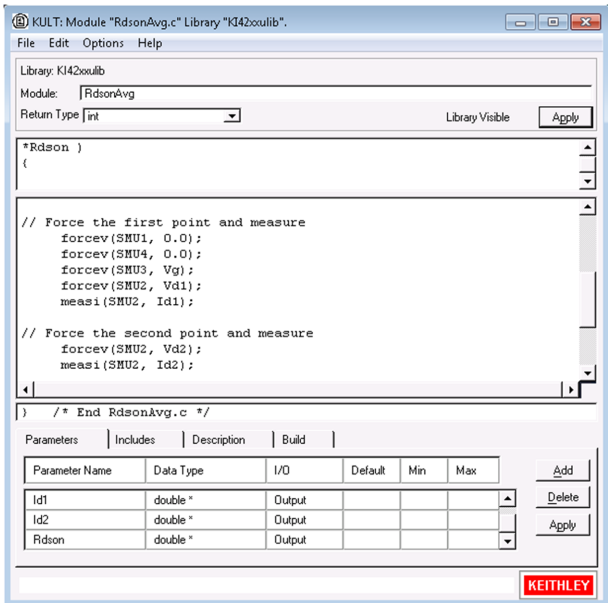
Figure 32: KULT module window
