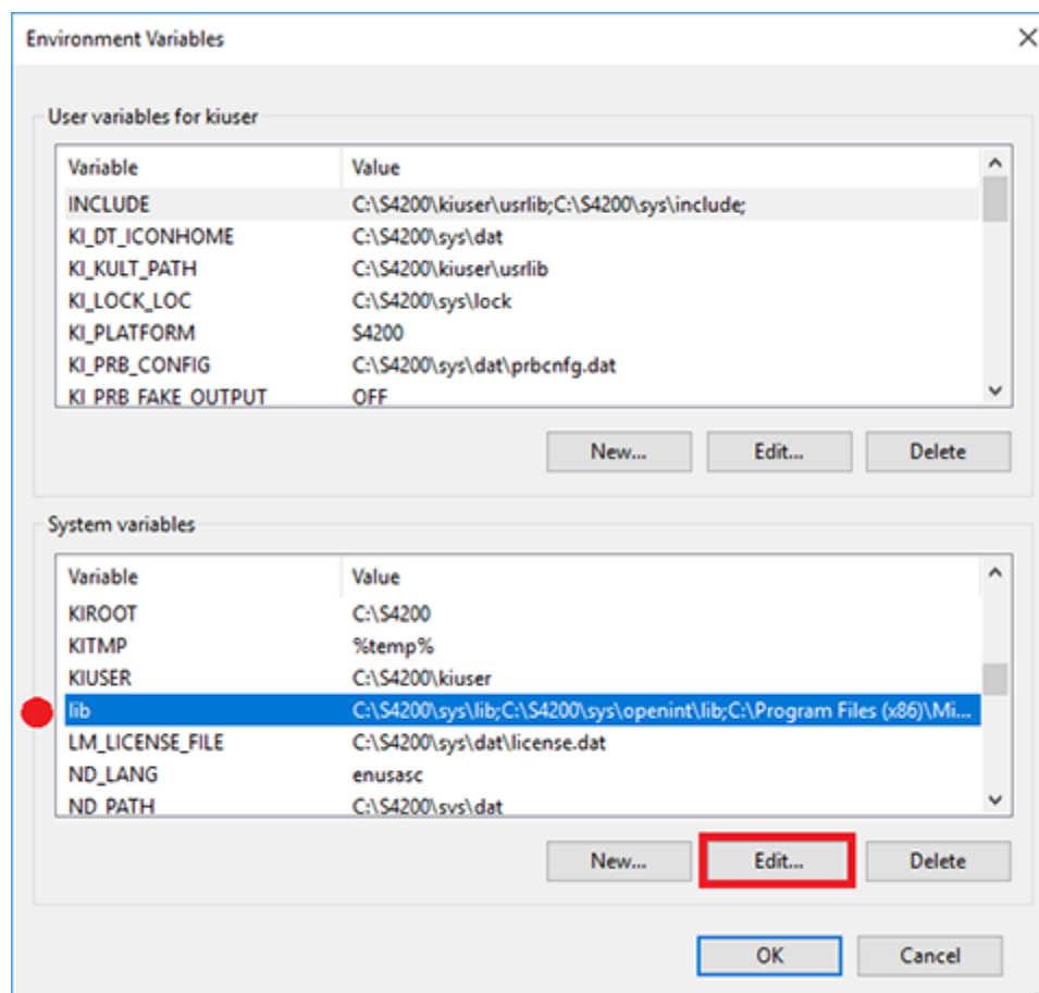
Figure 72: Enter environmental variables
