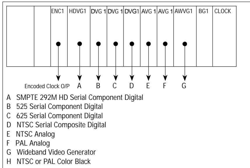
Figure 1. TG2000 configured to supply signals in several formats simultaneously.
