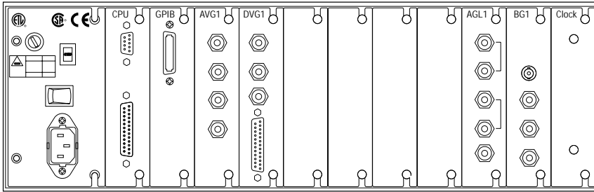
TG2000 Rear Panel.
